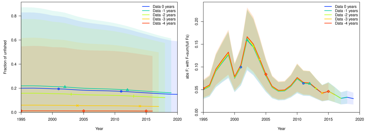
Figure 23: Retrospective patterns of relative spawning biomass and fishing mortality for the 2022 diagnostic case, compared with estimated uncertainty levels.
