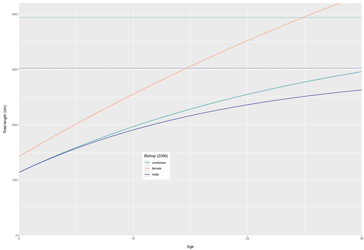
Figure 12: Comparison of growth curves for shortfin mako shark in the southwest Pacific Ocean used in the current assessment. Dashed lines show L_{\infty} for male and combined growth curves female L_{\infty} was estimated to be over 7m and is not shown in this plot.
