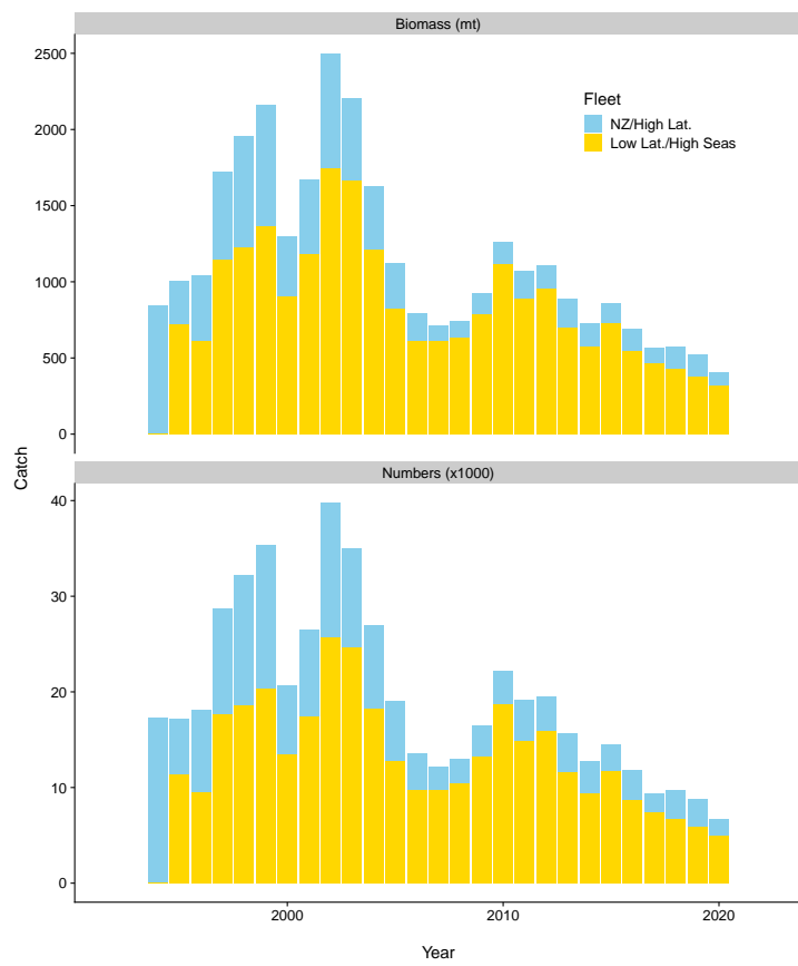
Figure 19: Catch by fleet in biomass and numbers.
