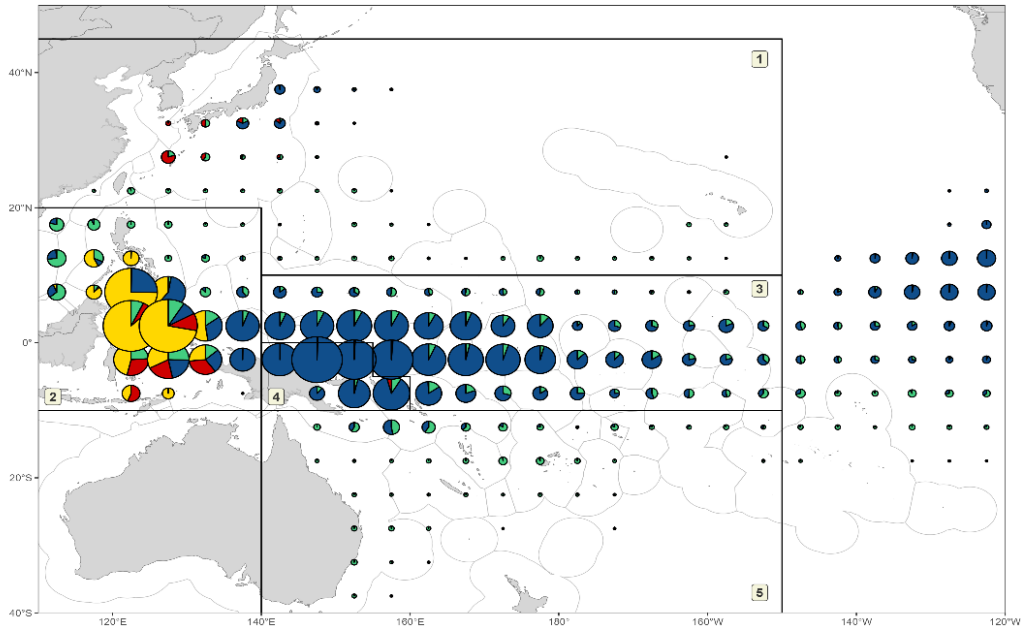
Figure 1. Distribution of yellowfin tuna catch by gear, 1990–2023 (longline - green; pole-and-line- red; purse seine - blue; other fisheries - yellow). The five-region spatial stratification used in stock assessment is shown.
