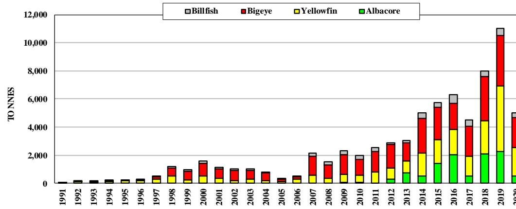
Figure 8. Catches by Federated States of Micronesia longliners
