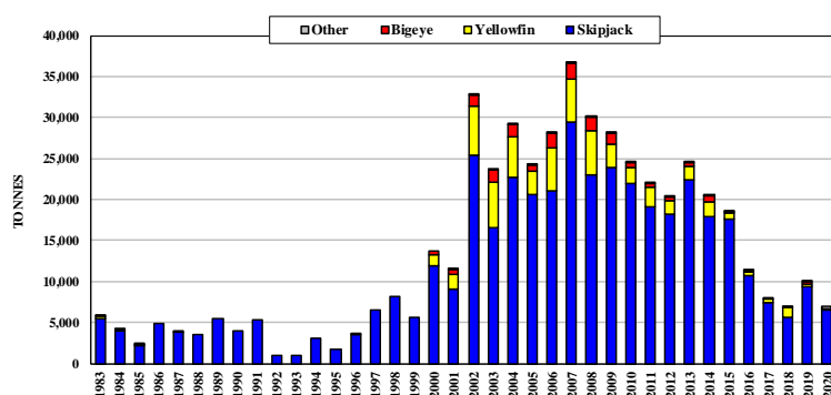
Figure 51. Catches by New Zealand purse seiners
