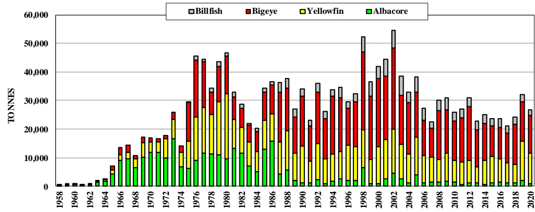
Figure 13. Catches by Korean distant-water longliners
