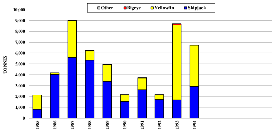
Figure 54. Catches by Russian purse seiners
