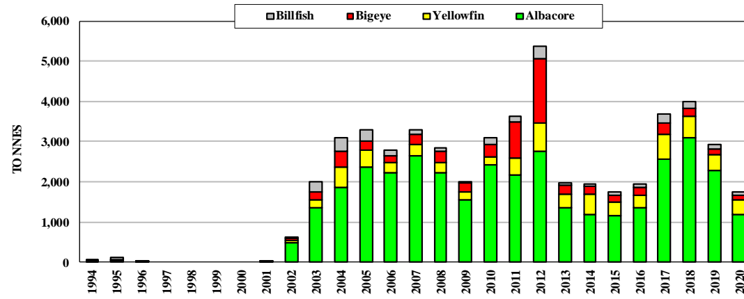
Figure 7. Catches by Cook Islands longliners
