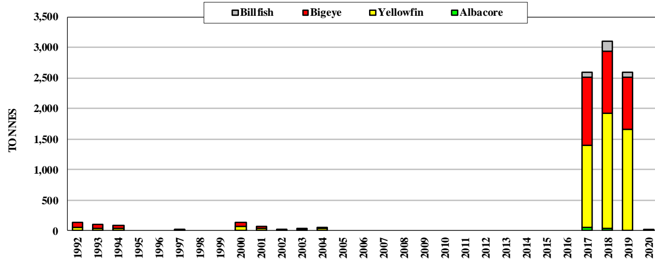
Figure 17. Catches by Palau longliners
