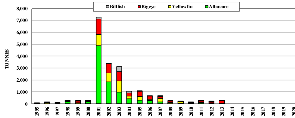
Figure 5. Catches by Belize longliners
