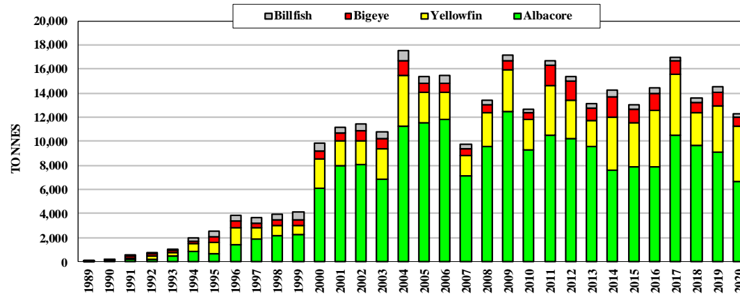
Figure 9. Catches by Fiji Islands longliners
