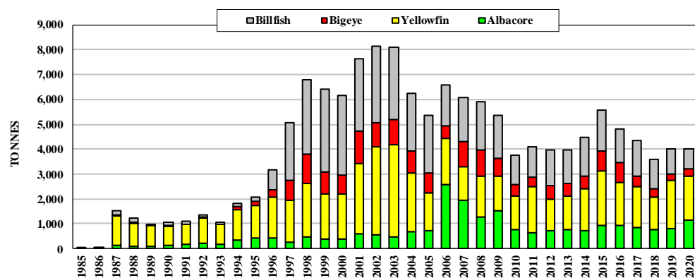
Figure 4. Catches by Australian domestic and chartered longliners
