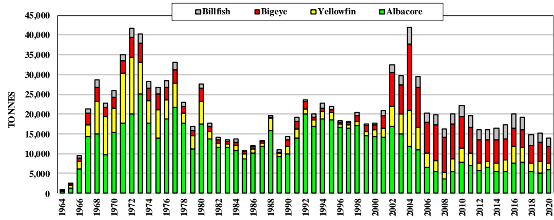
Figure 24. Catches by Chinese Taipei distant-water longliners
