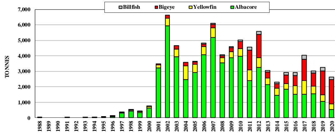
Figure 27. Catches by United States longliners based in American Samoa
