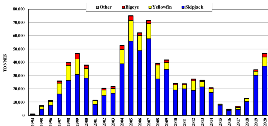
Figure 60. Catches (tonnes) by Vanuatu purse seiners
