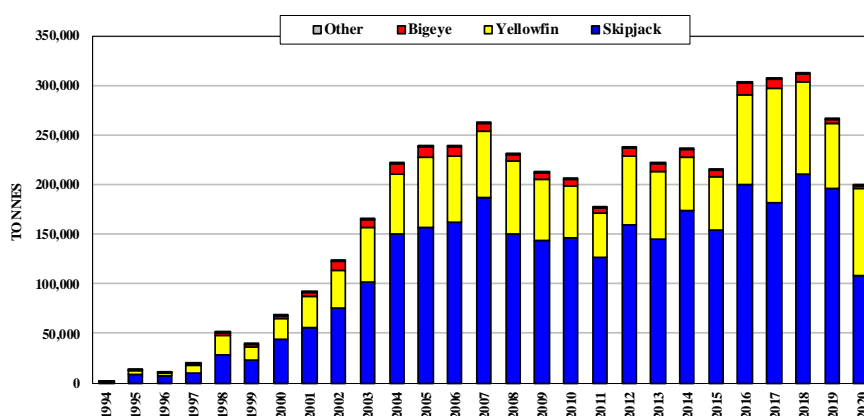
Figure 52. Catches by Papua New Guinea purse seiners
