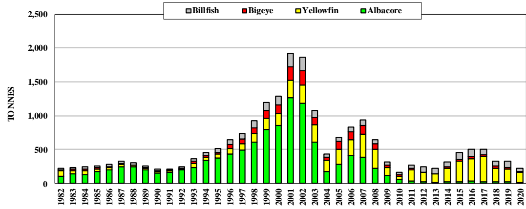
Figure 25. Catches by Tongan longliners
