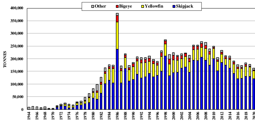
Figure 46. Catches by Japanese purse seiners
