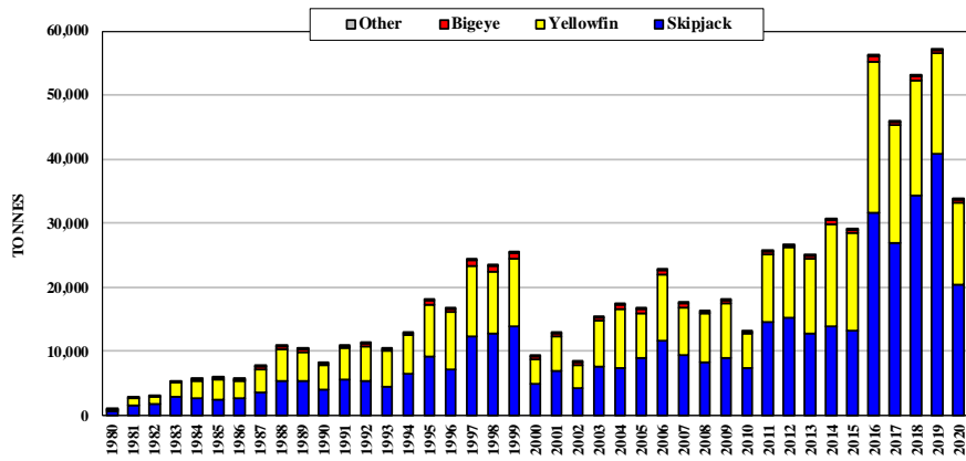
Figure 55. Catches by Solomon Islands purse seiners
