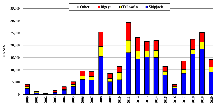
Figure 43. Catches by Ecuador purse seiners
