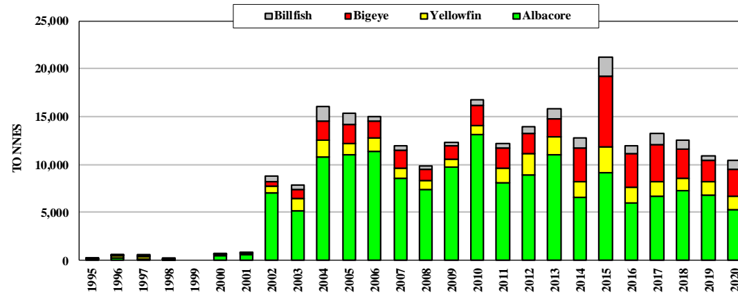
Figure 30. Catches by Vanuatu longliners
