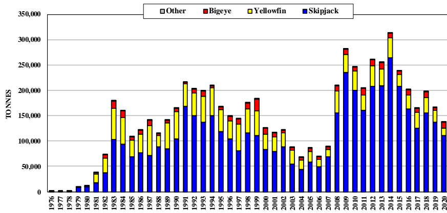
Figure 59. Catches by United States purse seiners
