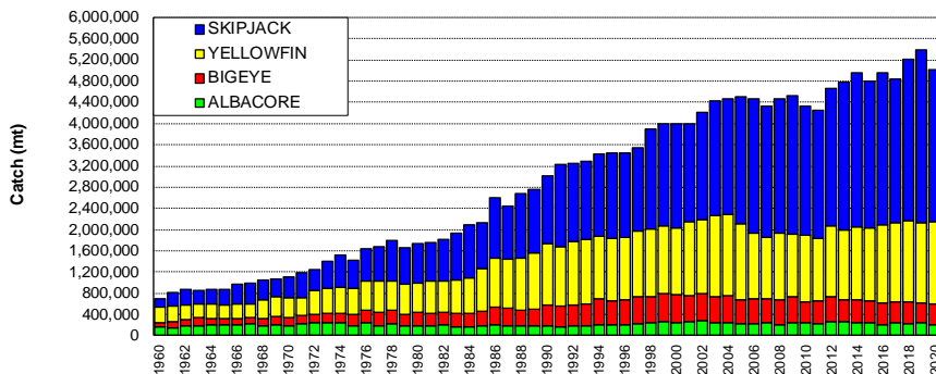
Figure 69. Global tuna catches, by species
