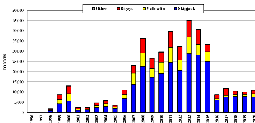
Figure 56. Catches by Spanish purse seiners
