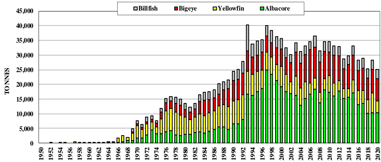
Figure 11. Catches by Japanese coastal longliners
