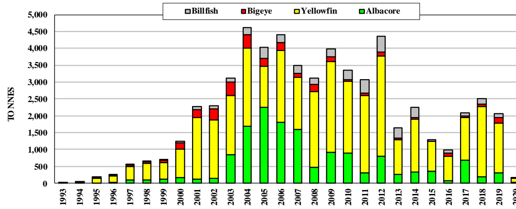
Figure 18. Catches by Papua New Guinea longliners
