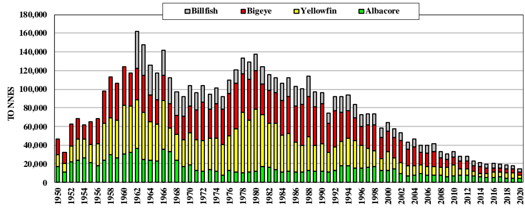
Figure 12. Catches by Japanese distant-water and offshore longliners
