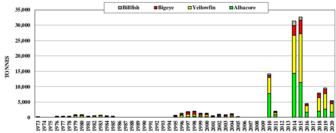
Figure 20. Catches by Solomon Islands longliners
