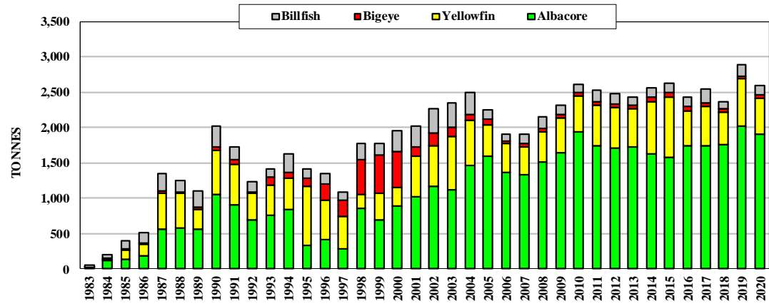
Figure 15. Catches by New Caledonian longliners
