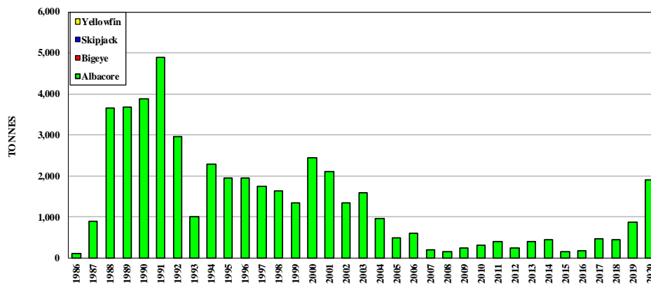
Figure 65. Seasonal catches of albacore by United States trollers in the South Pacific
