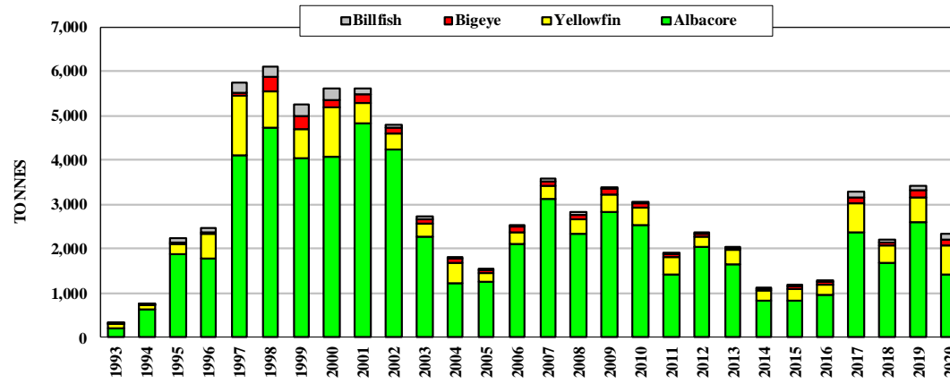
Figure 19. Catches by Samoan longliners
