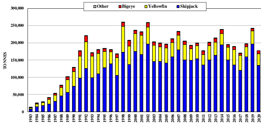
Figure 57. Catches by Chinese Taipei purse seiners
