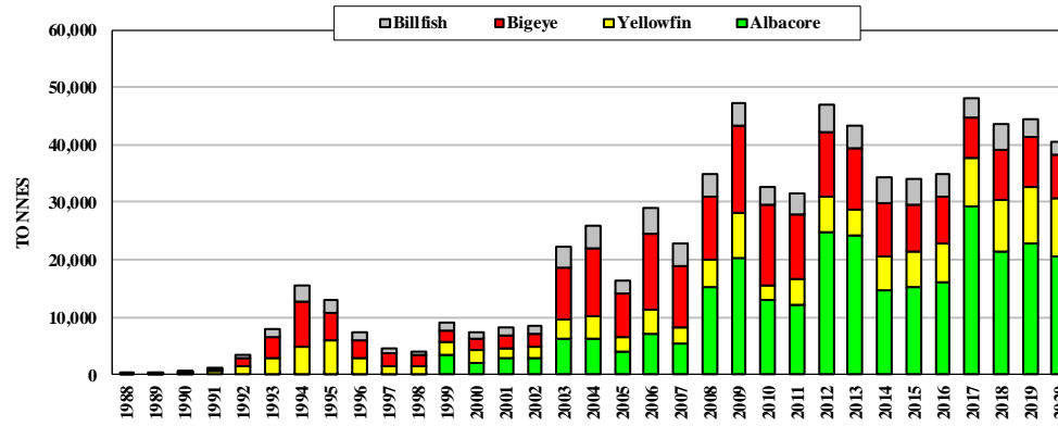
Figure 6. Catches by Chinese longliners
