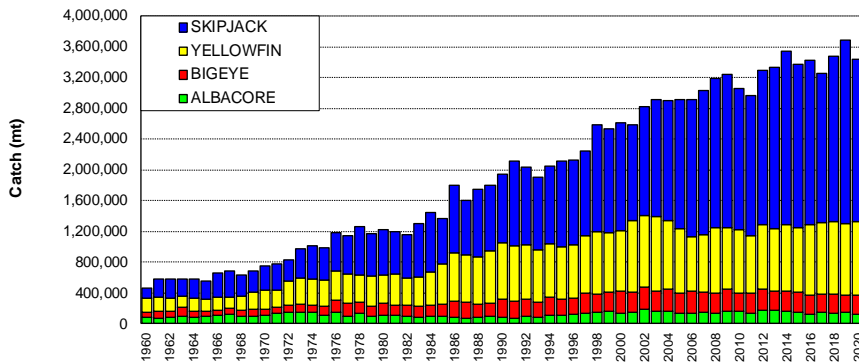
Figure 68. Catches in the Pacific Ocean, by species
