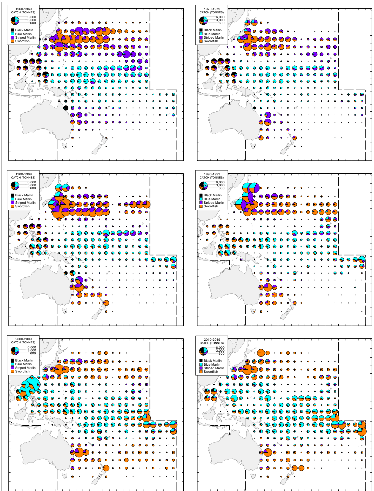
Figure 71. Distribution of billfish catch by species for the WCPFC LONGLINE fishery, by decade since 1960
