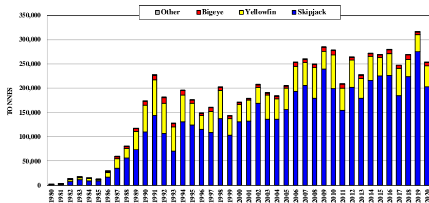
Figure 48. Catches by Korean purse seiners
