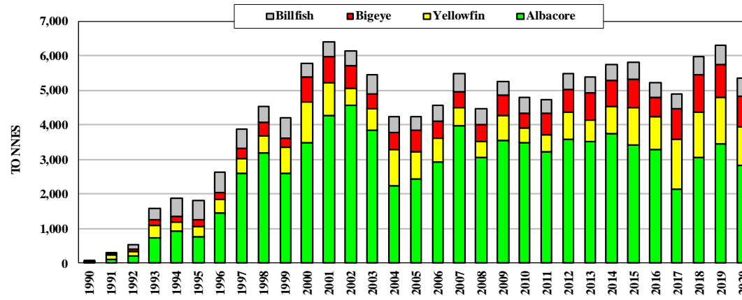
Figure 10. Catches by French Polynesian longliners
