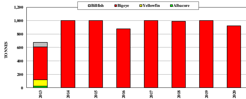
Figure 29. Catches by United States longliners based in Commonwealth of North Marianas Islands (CNMI)
