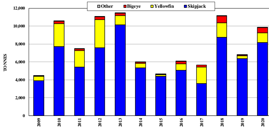
Figure 58. Catches by Tuvalu purse seiners
